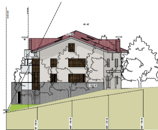
BATIMENT A - FACADE EST
